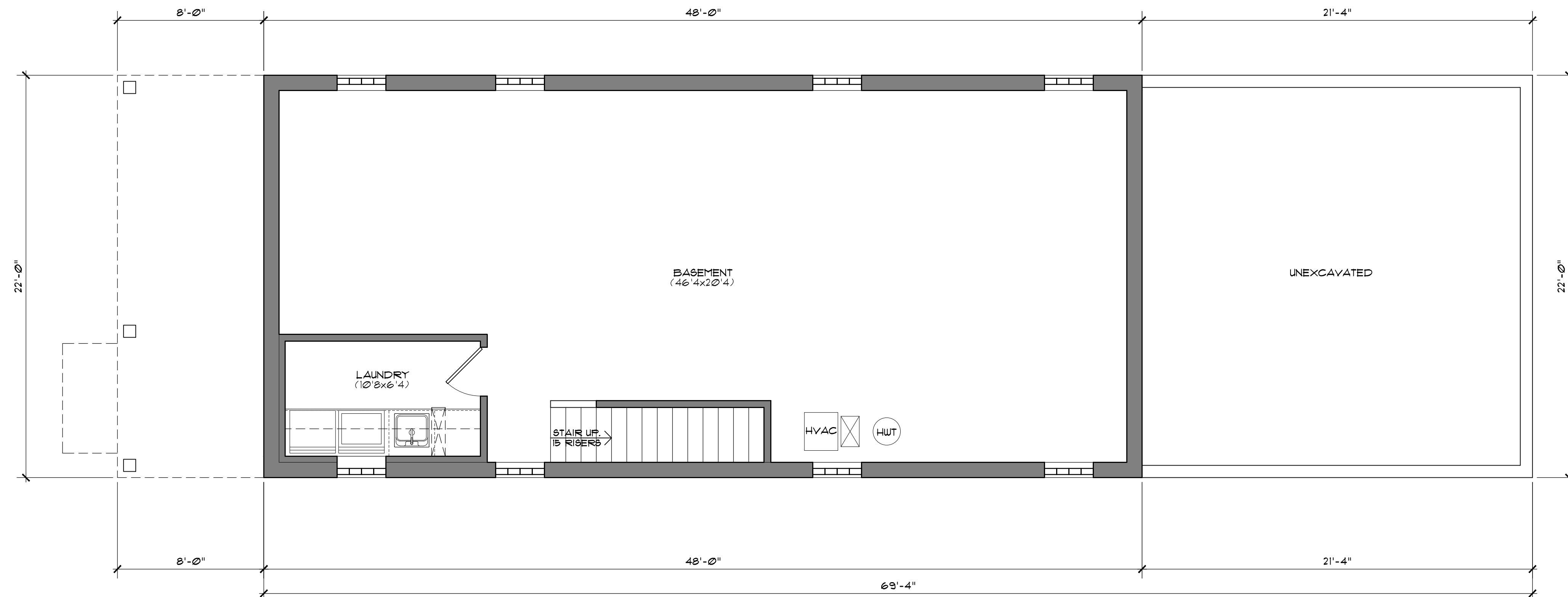
BASEMENT PLAN
