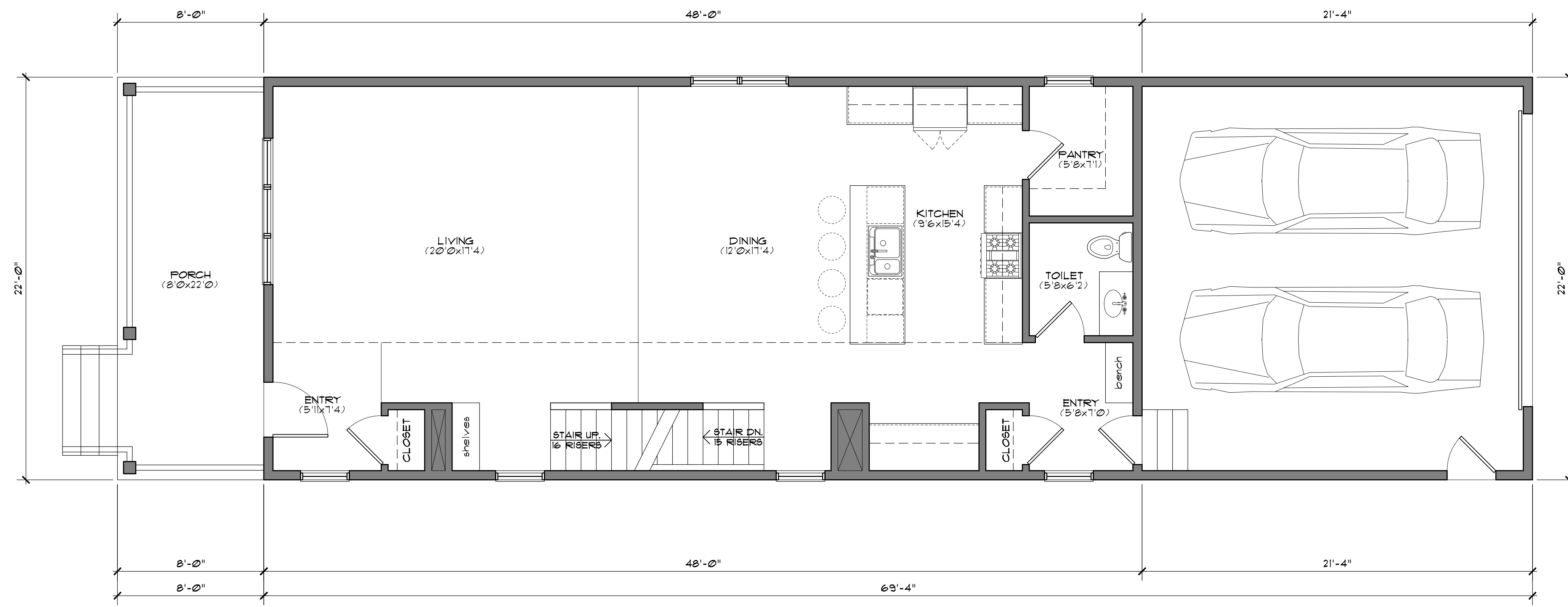
1ST FLOOR PLAN
