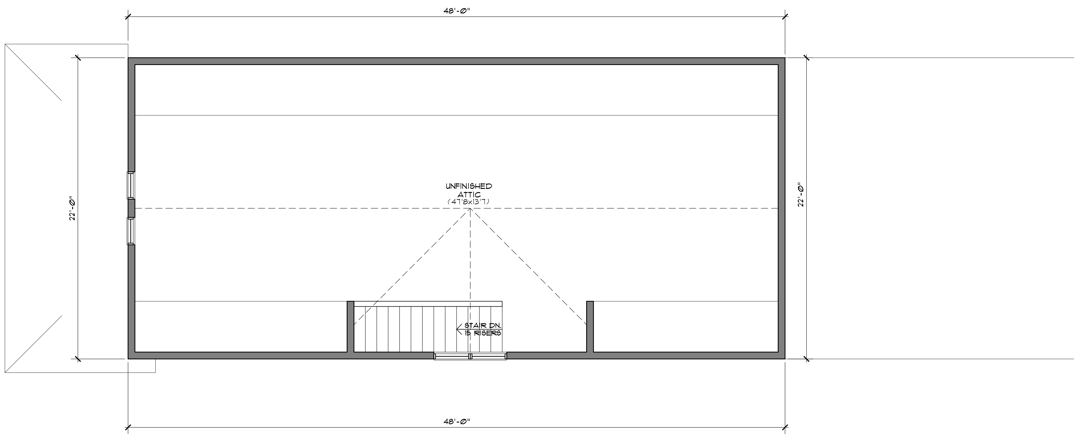
ATTIC PLAN
